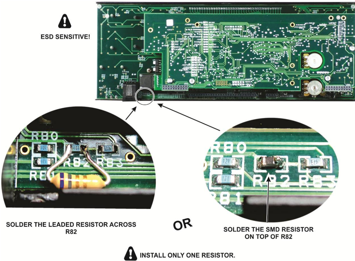
Figure 6. Installing Resistor Across R82.
